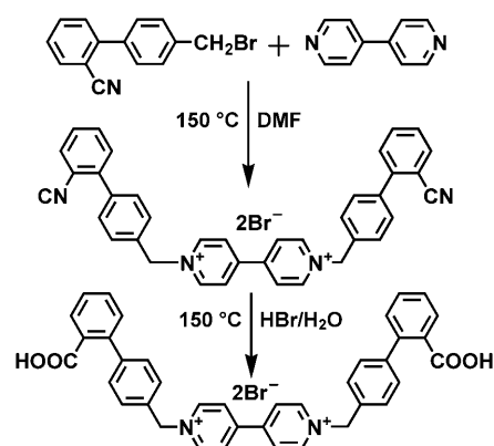
Scheme 1. Synthesis of the viologen derivative ( H_2Bcbpb )Br 2 .
